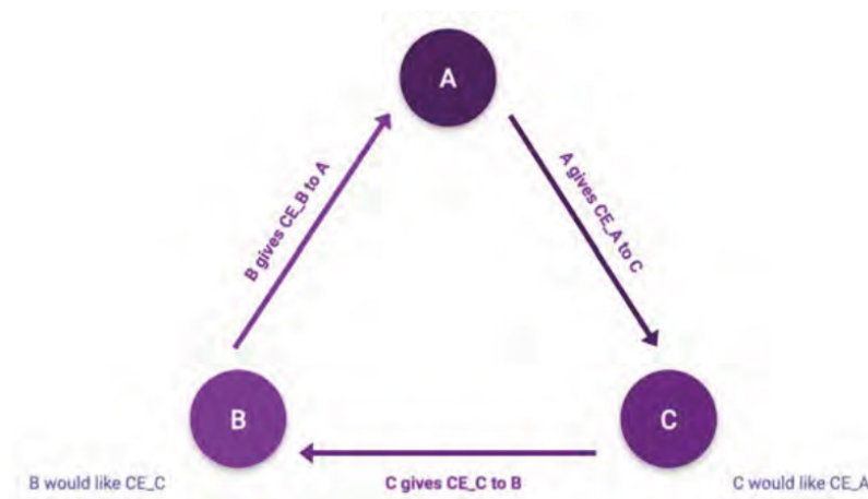
Figure 9 – Pairwise trade
